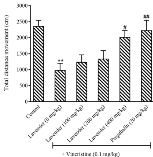
Fig. 1. Effect of Lavandula angustifolia (100, 200, and 400 mg/kg) on open field test in vincristine-induced neuropathic pain. Data are expressed as mean ± SEM, n = 8. ** P < 0.01 Indicate significance differences in comparison with the control group; # P < 0.05 and ## P < 0.01 versus vincristine-treated (lavender 0 mg/kg) group.
