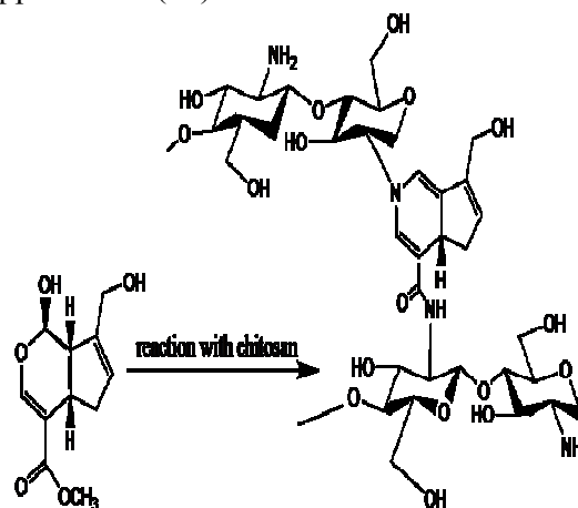
Fig. 4. Chemical cross-linking between chitosan chains in the presence of genipin.
